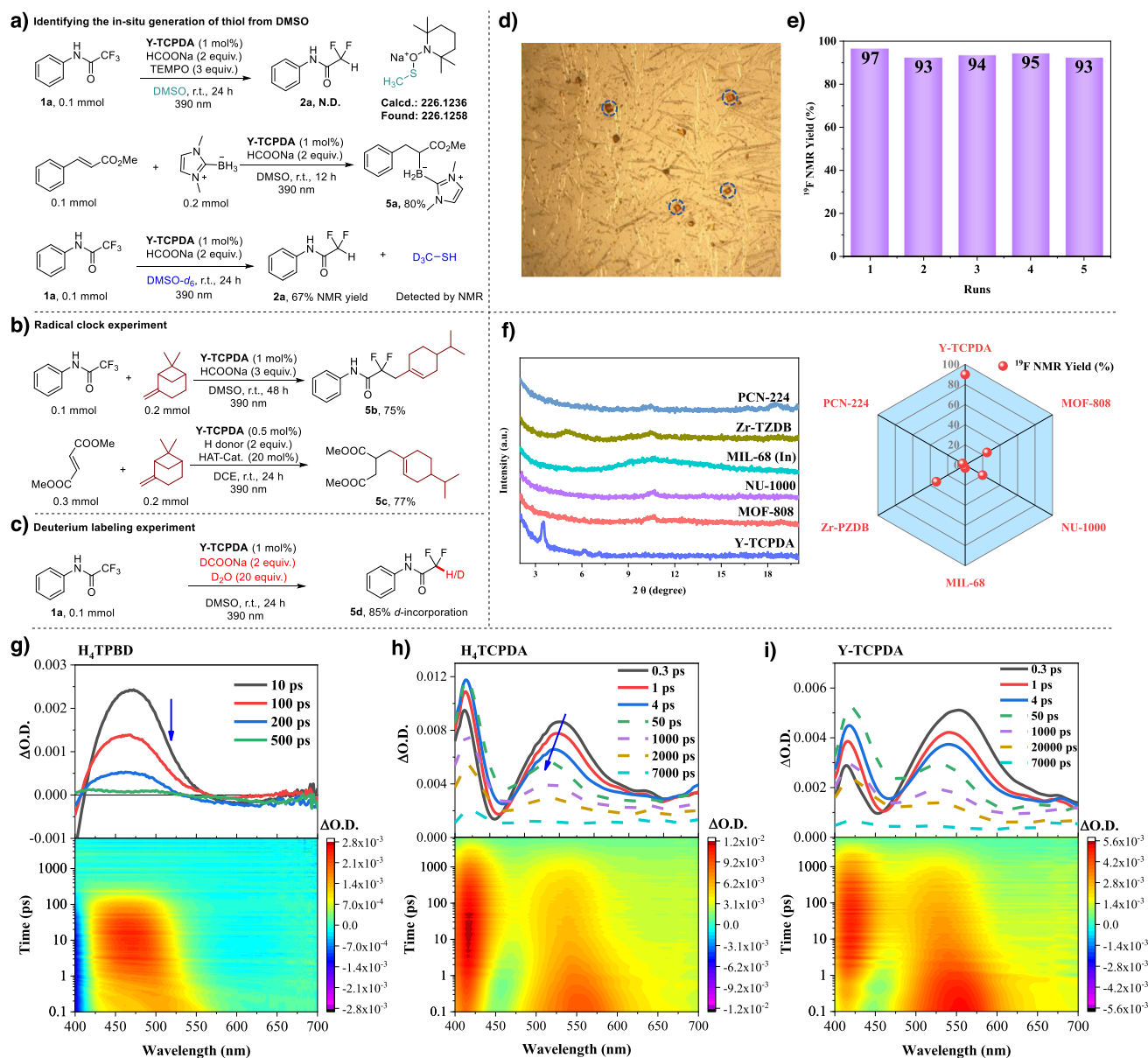
Figure 4. Mechanistic investigations. a) Experiments to illustrate the in-situ generation of CH_3SH from DMSO. b) Radical clock experiments. c) Deuterium labeling experiment. d) Figure of Y-TCPDA crystals (in blue cycle) after reaction. e) Recycle test, yields of 2a in 5 runs. f) Employment of other MOFs as the catalyst for defluorination and their stability evaluation after the reaction. g)–i) Transient absorption spectra of H_4TPBD g), H_4TCPDA h), and Y-TCPDA i) at selected pump-probe time delays, and the corresponding complete transient absorption surface probed; \Delta O.D. = difference in optical density; all TA spectra were recorded in DMSO following 390 nm excitation.
